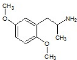
2,5-Dimethoxyamphetamine
